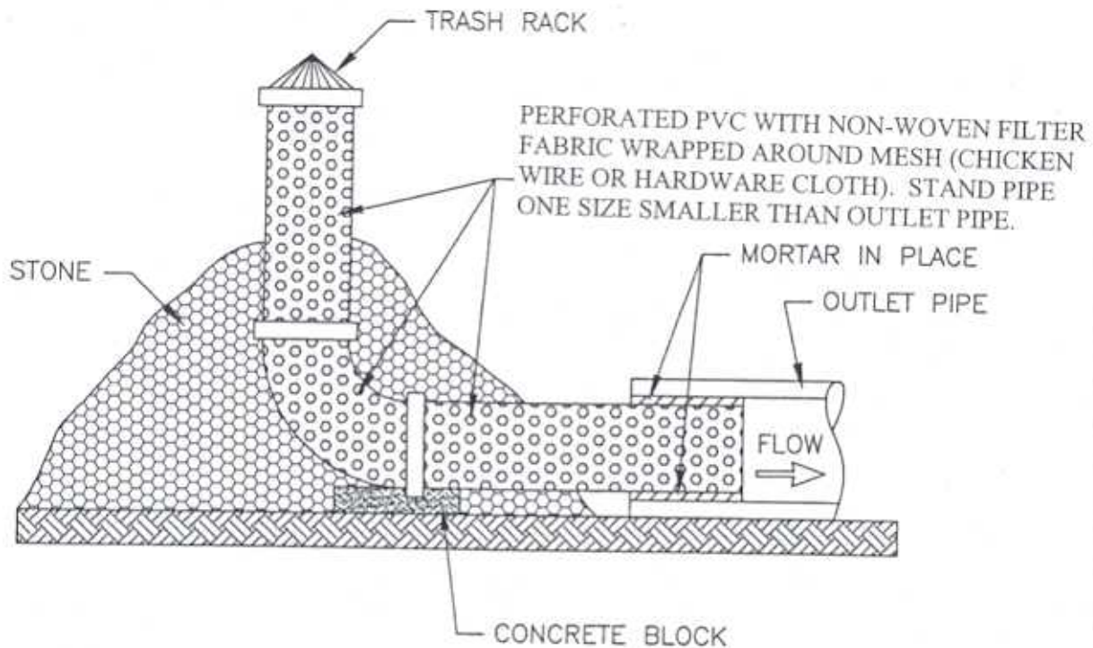
PERFORATED RISER DETAIL
