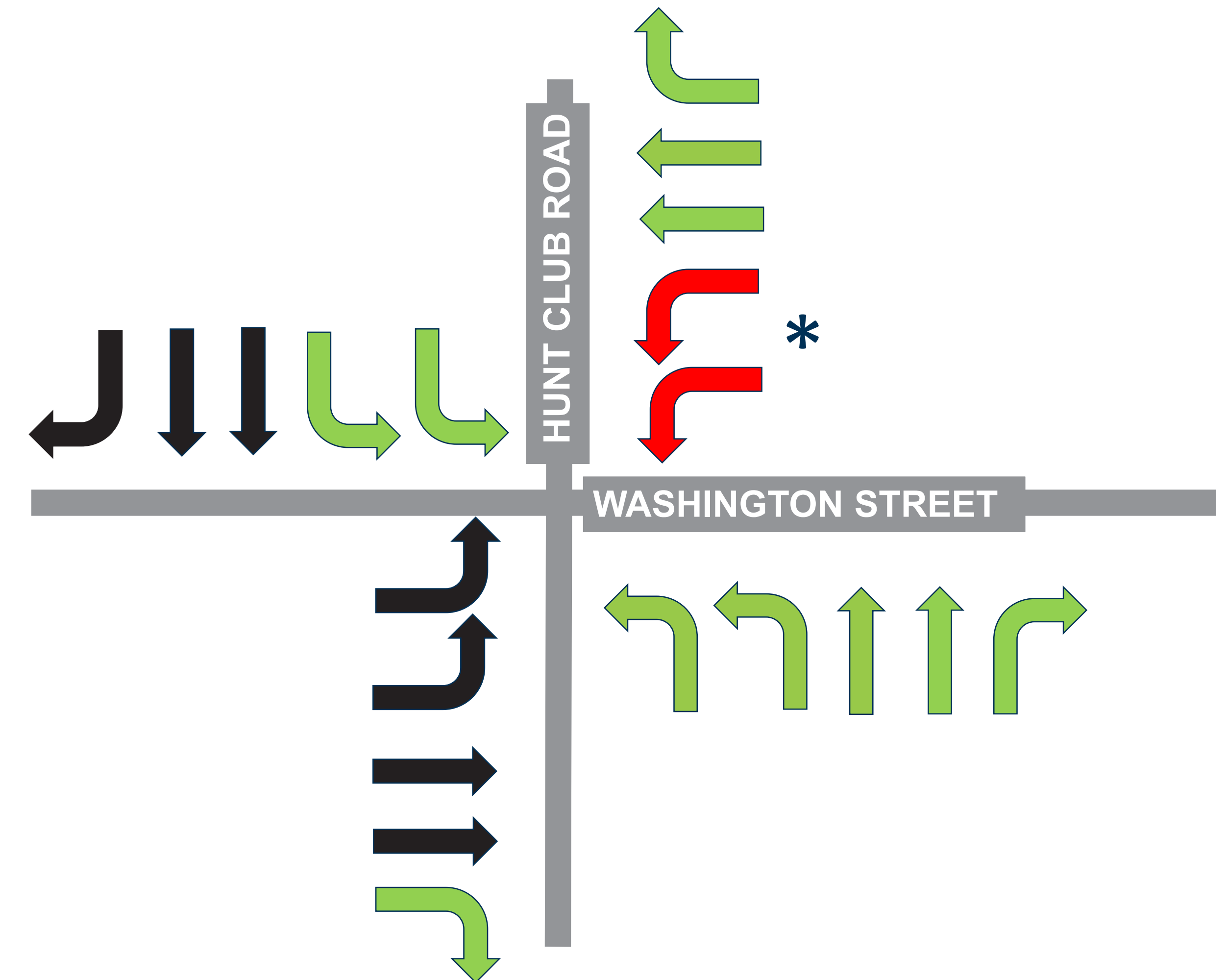
Proposed Improvements, Protected Left Only
