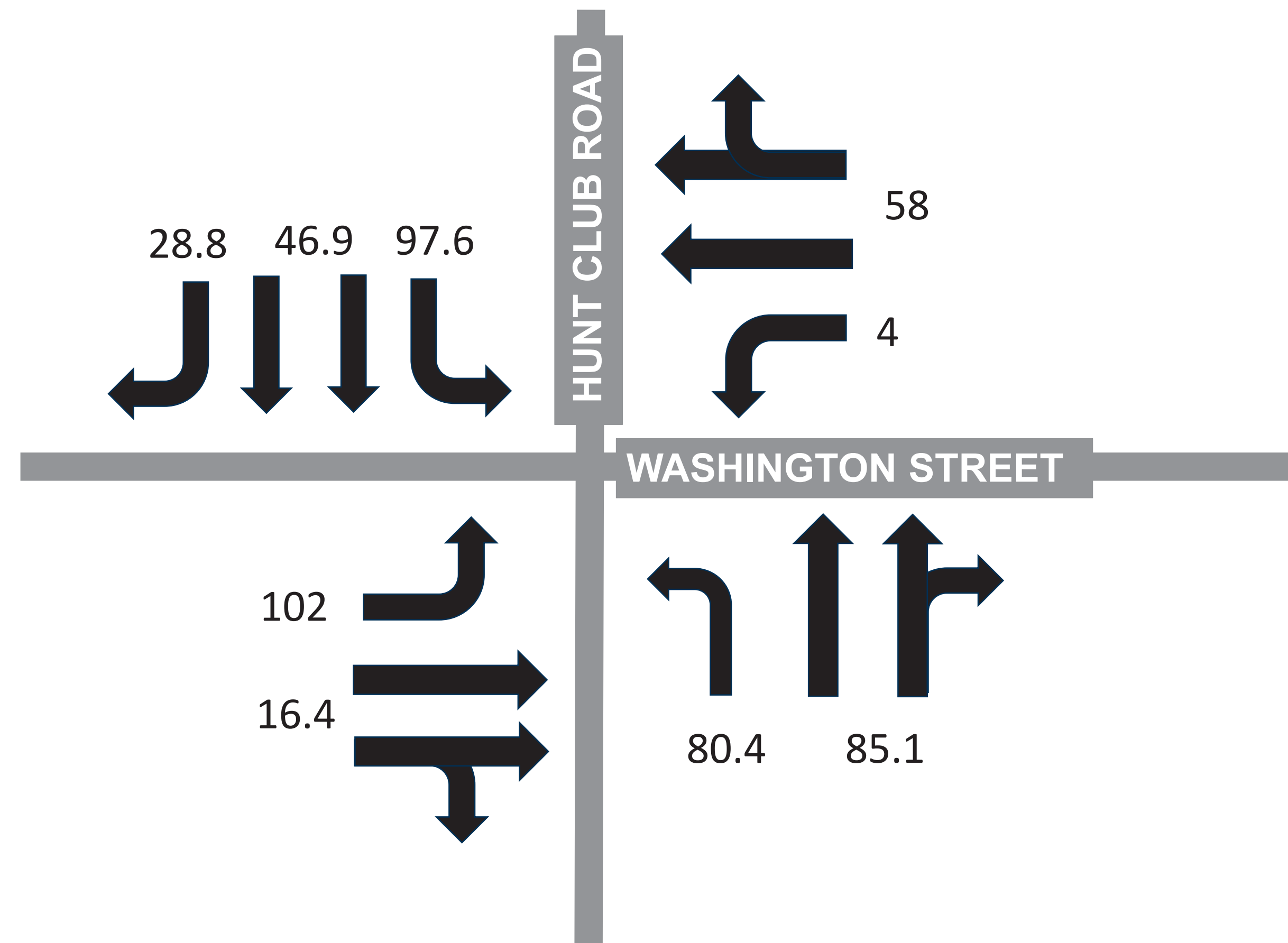
Existing Conditions (Permissive, Protected Left)
