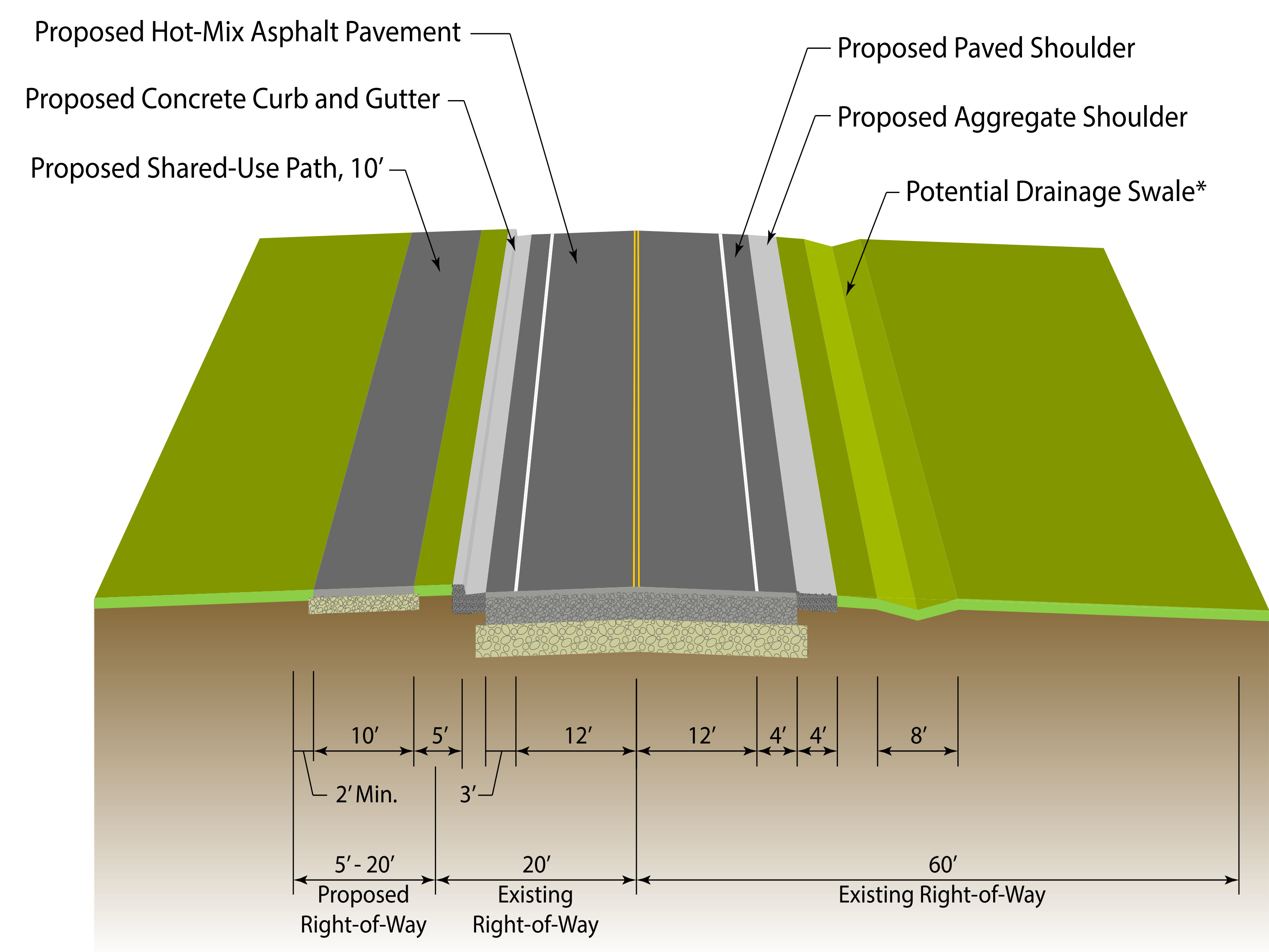
Proposed Typical Sections
