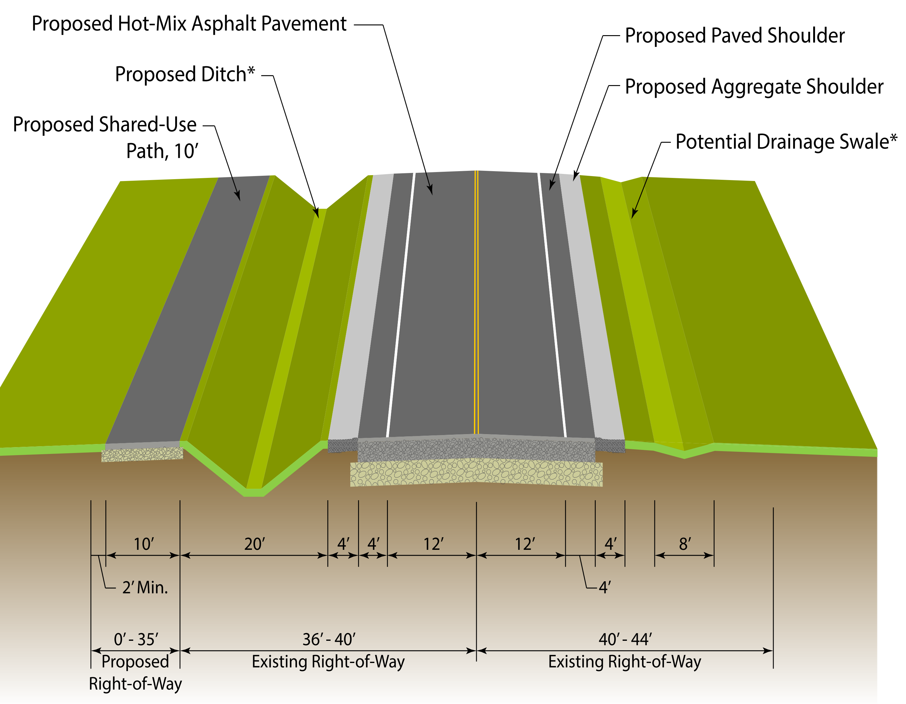
Proposed Typical Sections
