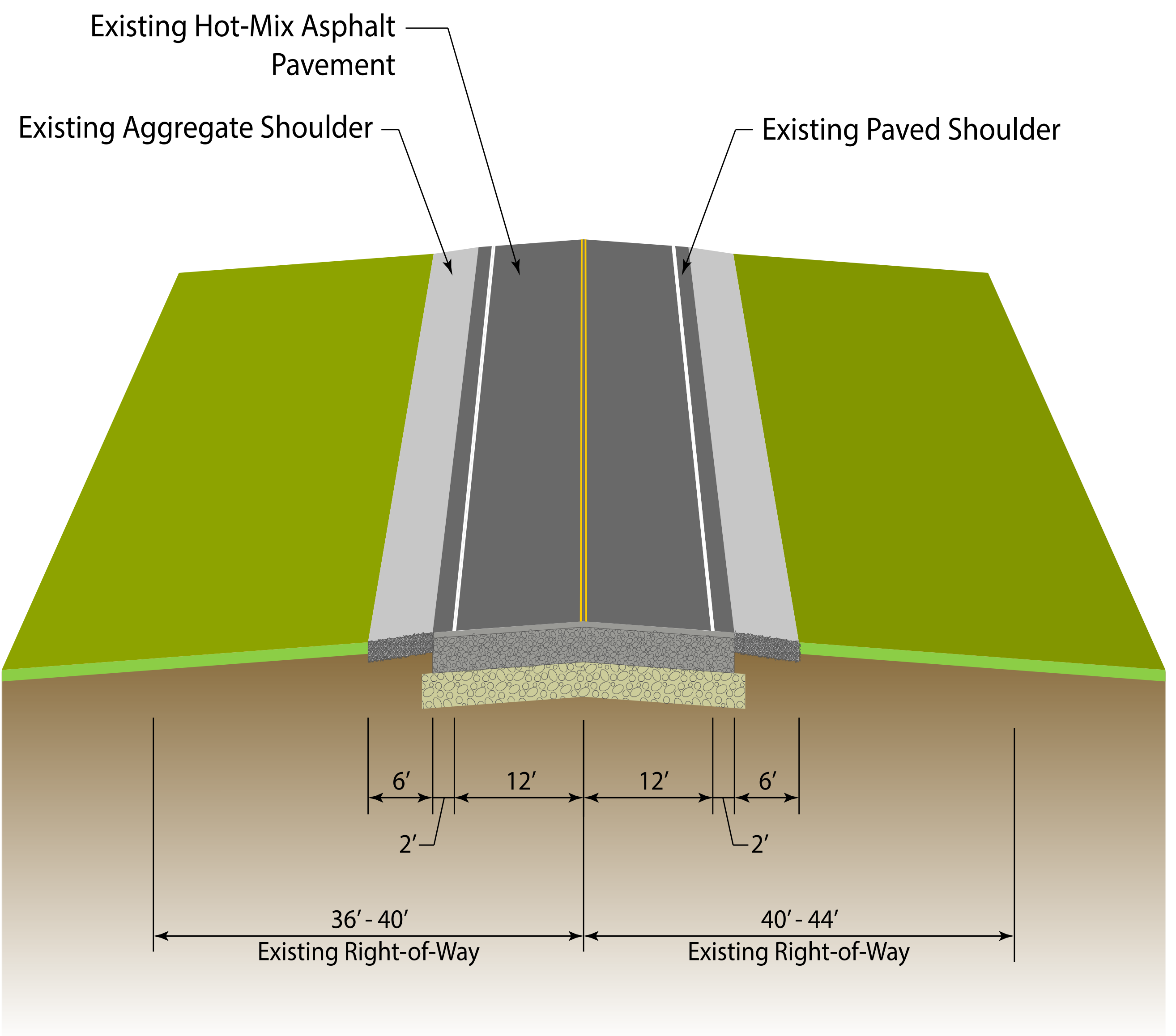
Existing Typical Sections
